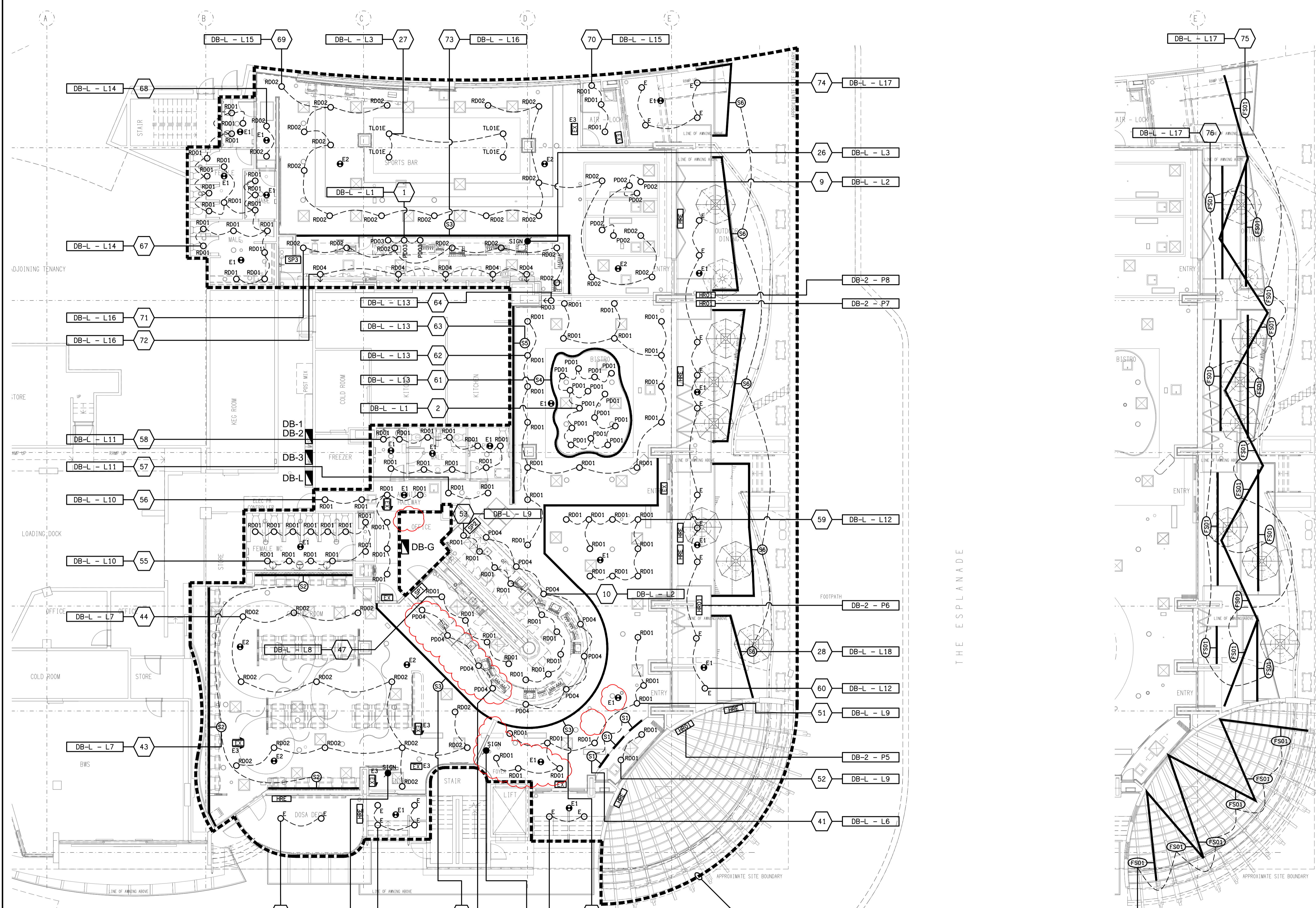
FESTOON LIGHTING REFLECTED CEILING PLAN SCALE 1:100
